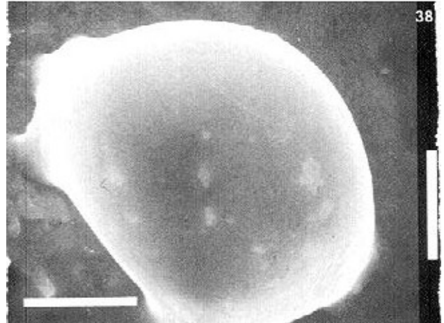
Figure 38. Object resert (SEM) from Hakatai Shale treated with HF. 26 x 35 \mu\text{m} . White bar—10 \mu\text{m} . Palynologist's discussion of this one: "38 appears to be covered with coating medium. I can't help very much with your friend's SEM images."
