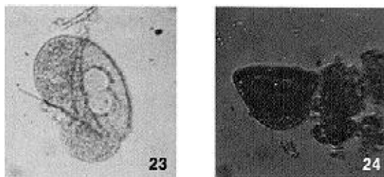
Figure 23. Hakatai shale sample p, Table II. Brownish-almost colorless. Clear. [34 x 53 \mu\text{m} ]. Saccate type. Note cell at top showing cell contents (nuclei?). Palynologist's discussion: "This is also a Pinus . You could be right about the nuclei. However, this would indicate that the pollen grain was very 'young.' Cytoplasm is never preserved in fossil material of the kind I work with."
