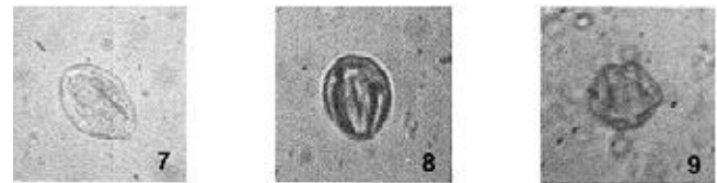
Figure 7. Hakatai shale sample m, Table II. [18 x 25 \mu m] Clear. Palynologist's discussion: "This almost certainly is a pollen grain—I would guess it is a tricolpate or tricolporate type. Unfortunately, this group is a large and difficult one and without a closer look I couldn't be certain what family is involved."
