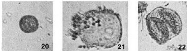
Figure 20. Hakatai shale sample p, Table II. Grey color, opaque. [19 \mu\text{m} diameter]. Palynologist's discussion: "Impossible to tell without more resolution."
