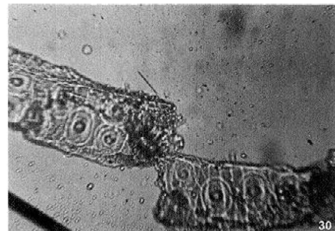
Figure 30. Hakatai Shale sample p, Table II. A tracheid with bordered pits. Tracheid width 51 \mu\text{m} . Width of bordered pit 26 \mu\text{m} . Width of pore in center of pit 6 \mu\text{m} . Length of tracheid 294 \mu\text{m} . Palynologist's discussion: "You are correct, these are tracheids. The bordered pits suggest that gymnosperms are involved."
