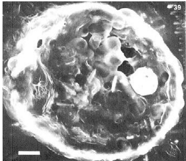
Figure 39. Object present (SEM) from Hakatai Shale treated with HF. [80 x 70 \mu\text{m} ]. White bar—10 \mu\text{m} . Palynologist said this looked somewhat like a charred carbon particle.
