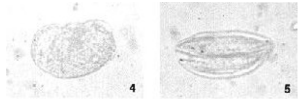
Figure 4. Hakatai shale, sample m, Table II. [25 x 56 \mu m] Clear. Palynologist's discussion: "Probably the same as Figure 3. As you suspect one of the bladders has been lost."
