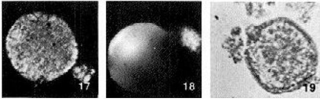
Figure 17. Hakatai shale sample p, Table II. Sidelight (darkfield) picture. Bright green color, speckled with yellow. Opaque. Granular surface. [40 \mu\text{m} diameter]. Palynologist's discussion: "This object is not a pollen grain. Fresh pollen is usually yellow in color and although the cytoplasm may be visible in untreated material, it does not look like the object on the photograph. My guess is that this is an algal cell."
