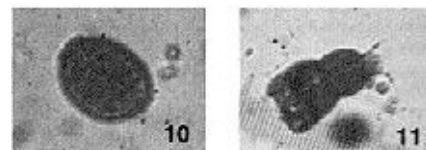
Figure 10: Hakatai shale sample m, Table II. [22 x 29 \mu m] Dark orange coloration, clear. Palynologist's discussion: "This could be a pollen grain but again identification is impossible because of poor resolution of the photograph."
