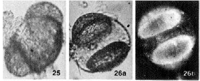
Figure 25. Hakatai shale sample p, Table II. Yellowish-brown color. Cloudy. [50 x 76 \mu\text{m} ]. Saccate type pollen. See caption Figure 24 for discussion.
